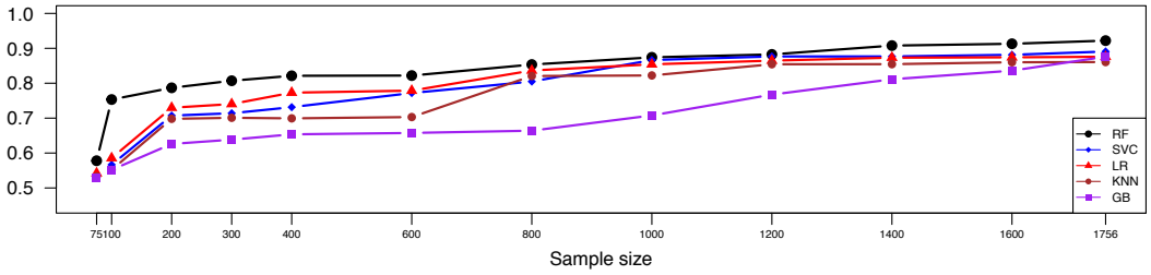
(a) Weighted AUC
