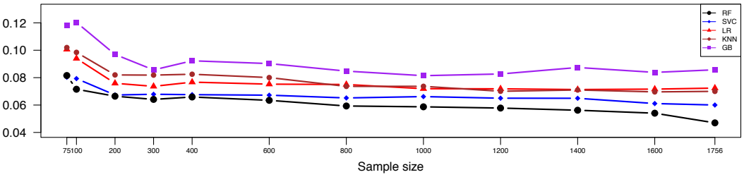
(c) Brier score
